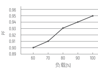
PF vs 负载
