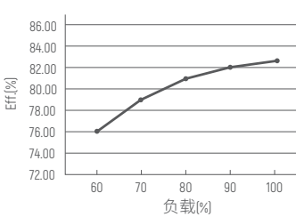
Eff. vs 负载
