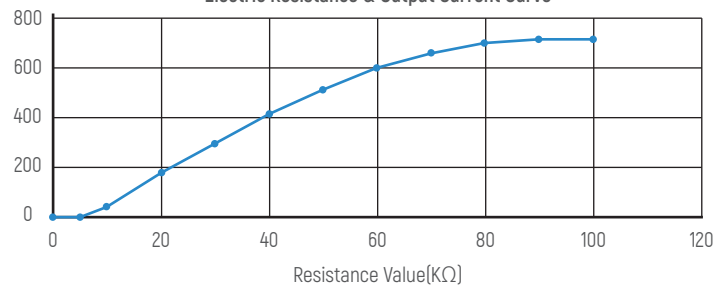
Electric Resistance & Output Current Curve
