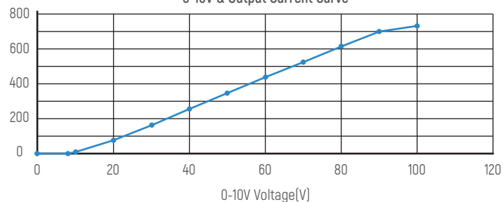
0-10V & Output Current Curve
